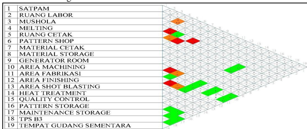
Gambar 2. Diagram ARC
