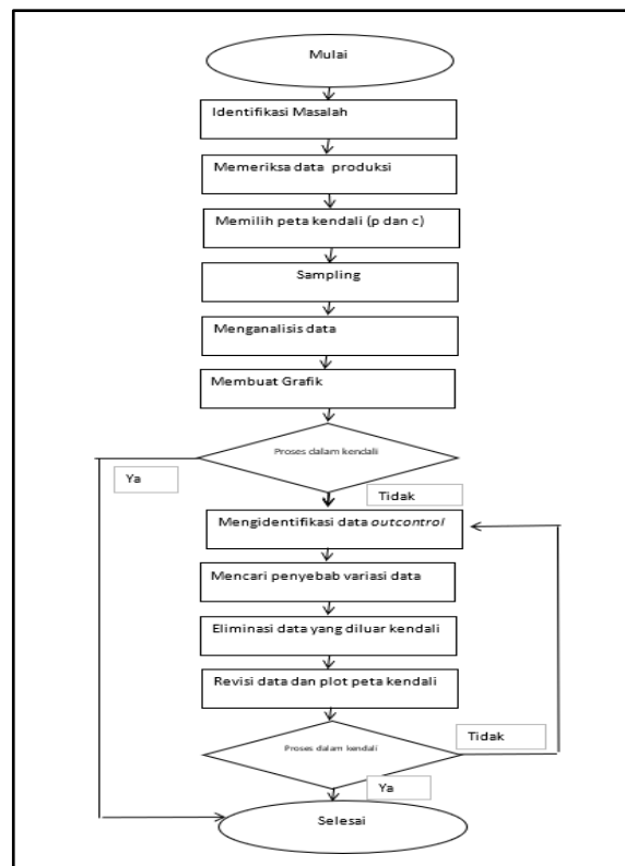
Gambar 3. Flowchart Penelitian
