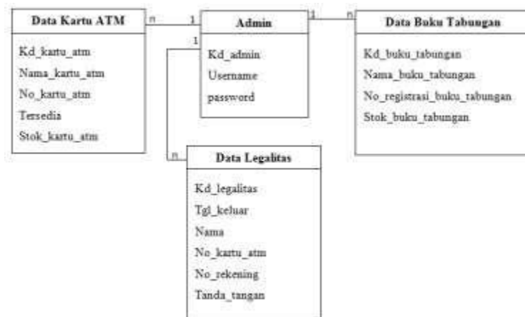
Gambar 3. Class Diagram
