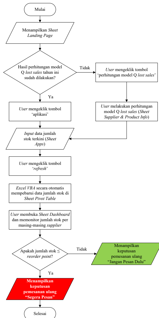
Gambar 7. Flowchart logika keputusan
