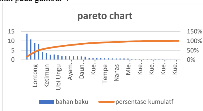
Gambar 5. Diagram Pareto
