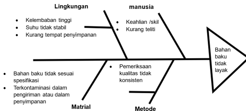
Gambar 7. Diagram Fishbone
