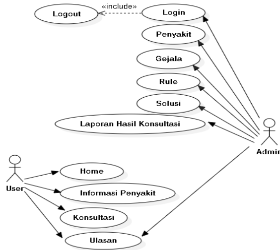
Gambar.1 Usecase diagram
