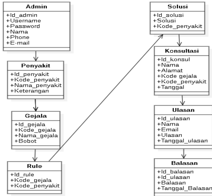
Gambar.4 Class Diagram
